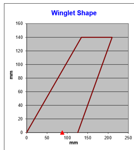
Note: Red Triangle is Aerodynamic Center (AC) of the Tiplet
