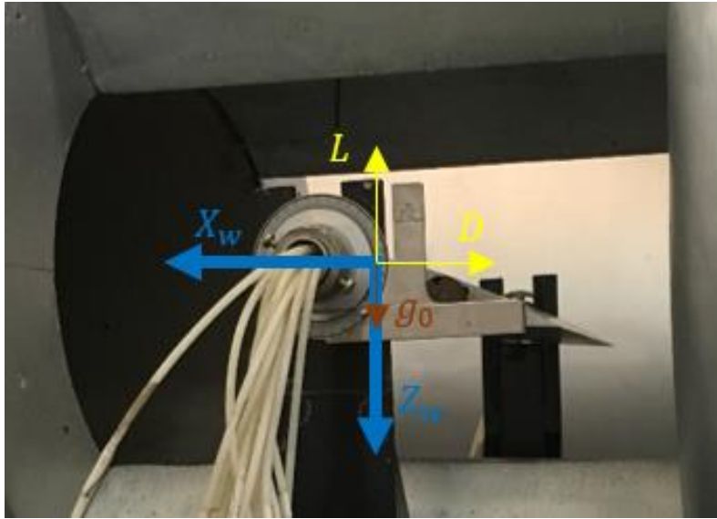
Figure 8 - Wind tunnel test section with wind axis and forces.
