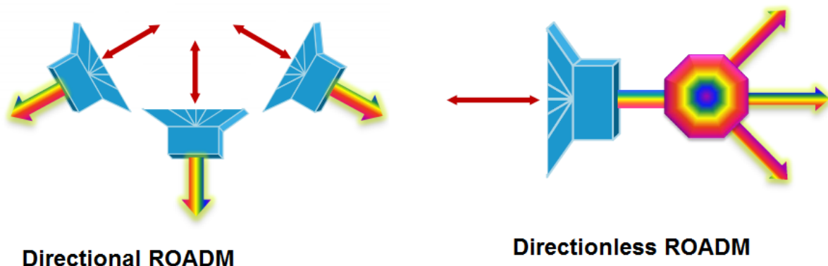
Slika 4.23. Directionless ROADM, [25]
