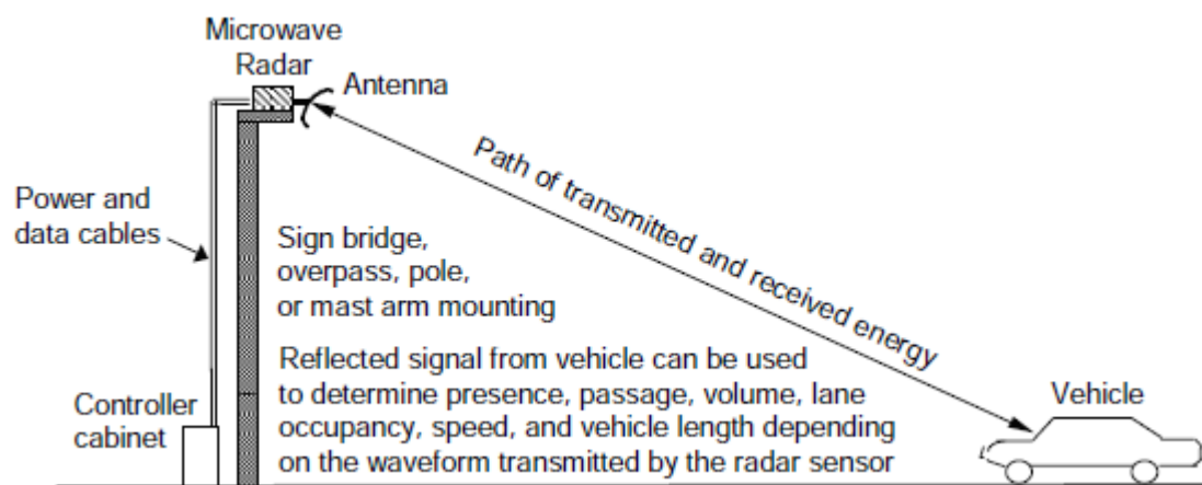
Figure 4 Microwave radar (source: Traffic sensor handbook, April 2016)
