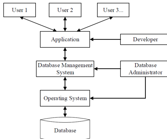
Figure 3.7: The composition of a database system [18]
